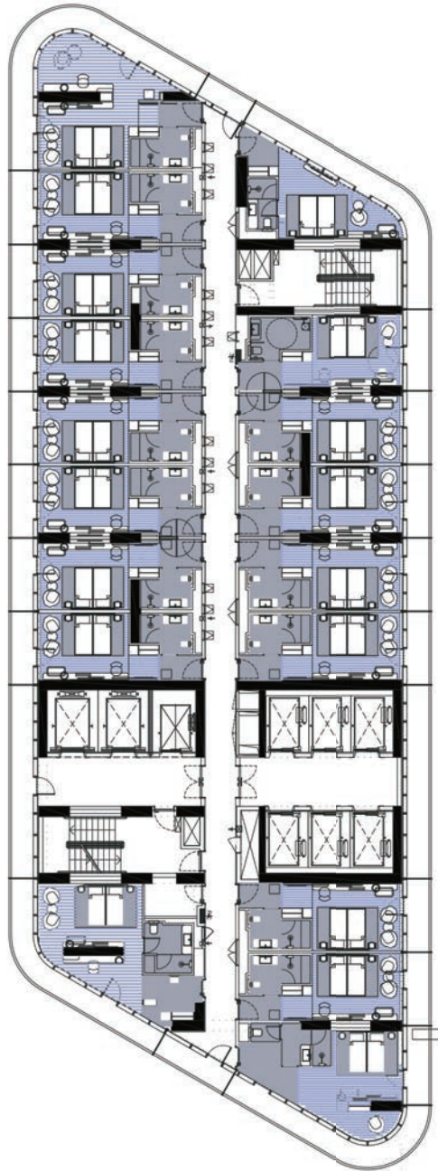
Typical 18 Room Floor Plate
